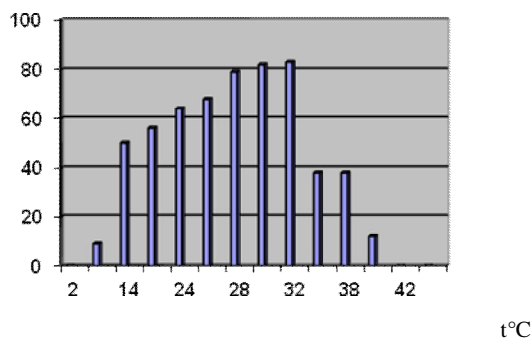
Fig. 1- Alternaria brassicae conidions' germination depending on temperature
